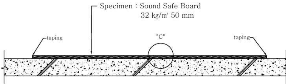
B-B' SECTION
